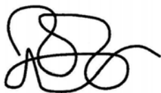
Linear random coil
