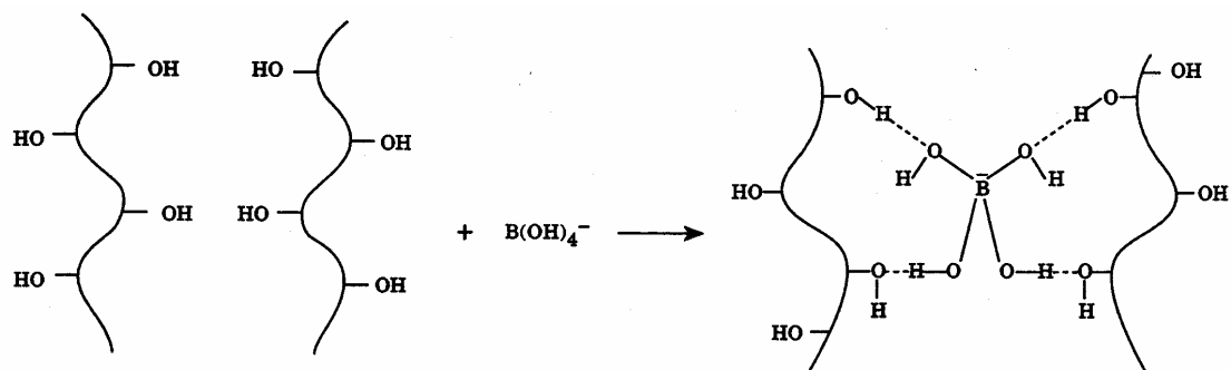
Figure 2. Structure of “slime”
